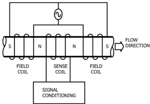
FIG. 3 Sensor Major Components
