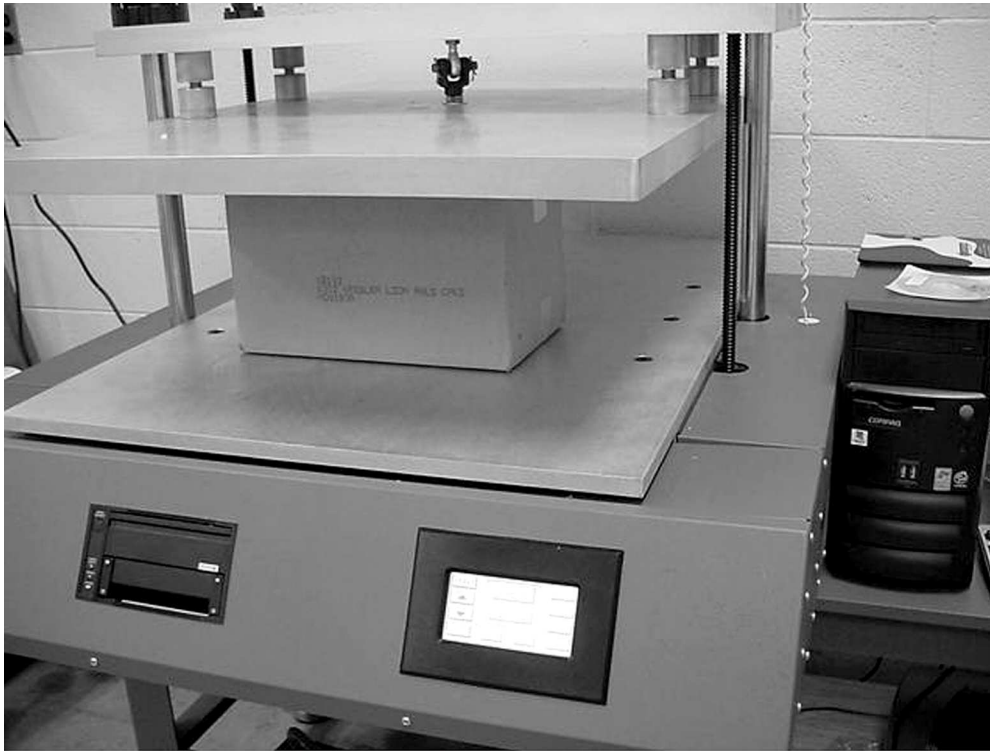
FIG. 3 Container Under Constant Load in Compression Test Machine With Fixed Platen
