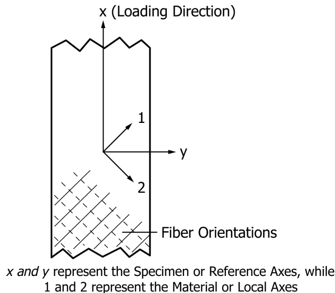
FIG. 2 Definition of Specimen and Material Axes
