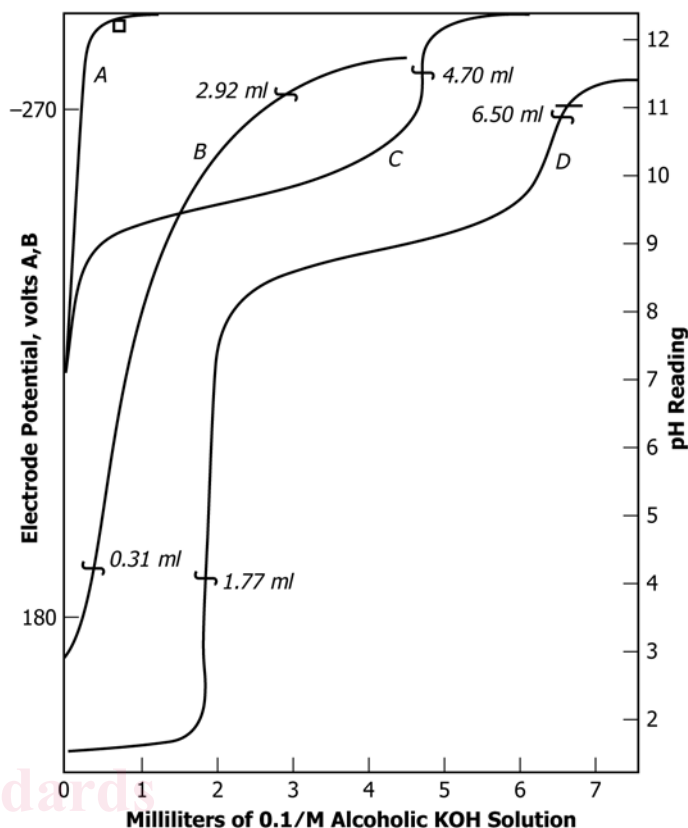
Key: Curve A—Blank on 125 mL of titration solvent. Curve B—10.00 g of used crankcase oil plus 125 mL of titration solvent. Since no sharp inflections are apparent, the end points are chosen at the meter readings obtained with the two aqueous buffer solutions. Curve C—10.00 g of oil containing a weak acid plus 125 mL of titration solvent. The end point is chosen as the point at which the curve is most nearly vertical. Curve D—10.00 g of oil containing weak and strong acids plus 125 mL of titration solvent. The end points are chosen as the points at which the curve is most nearly vertical.
