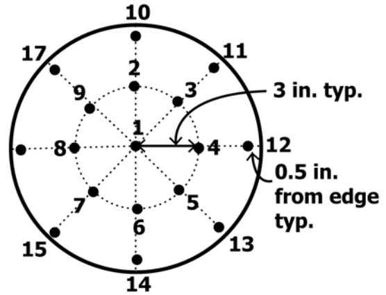
FIG. 1 Thermocouple Placement
