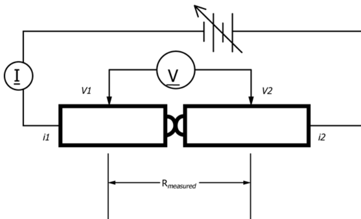
FIG. 1 Schematic Representation of 4 Wire Measurement Circuit
