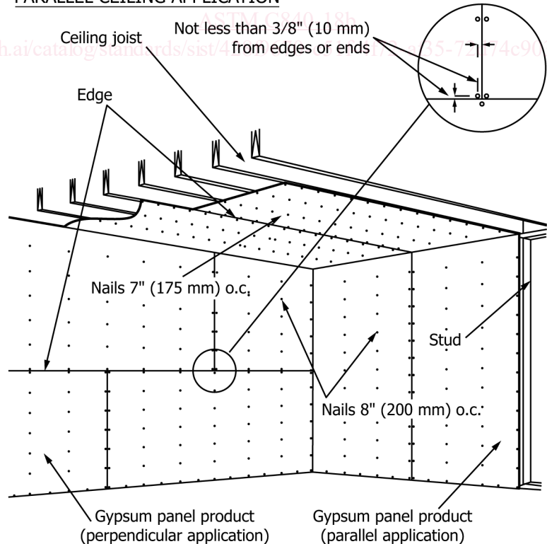
FIG. 2 Single Nailing
