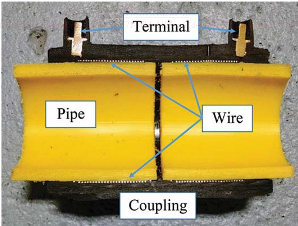
FIG. 1 Typical Cross-Sectional View of an Electrofusion Coupling Joint
