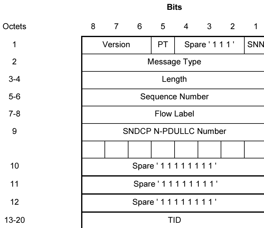
Figure 2: Outline of GTP header (standards.iteh.ai)
