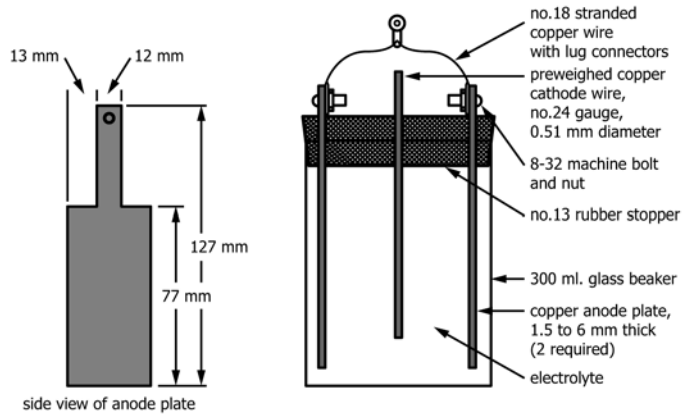
FIG. 2 Copper Coulometer
