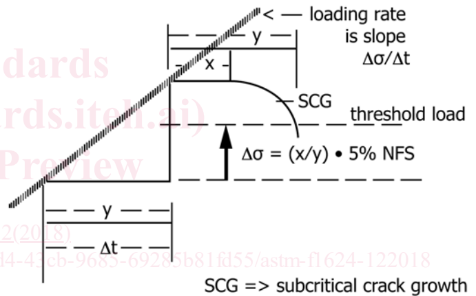
FIG. 5 Extrapolation Method for Type A Threshold Load Determination
