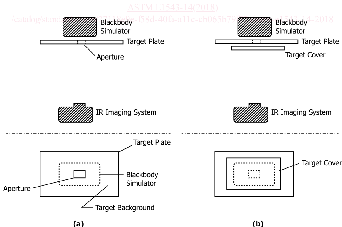
FIG. 1 Schematic of NETD Procedure Configuration; (a) When Measuring Signal and (b) When Measuring Noise
