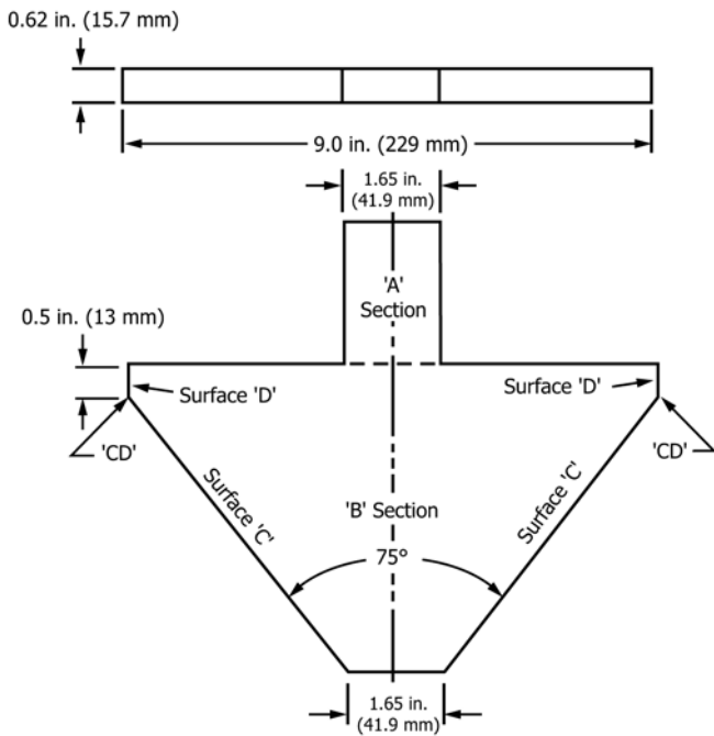
FIG. 4 Test Probe for Partially Bounded Openings
