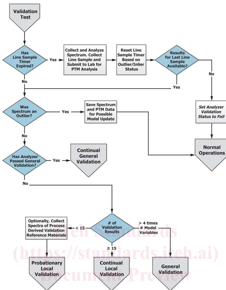
FIG. 3 Flowchart of Process Analyzer Validation Practice General Validation Validation Test
