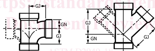
SANITARY TEE Single & Double 45° WYE Single & Double
