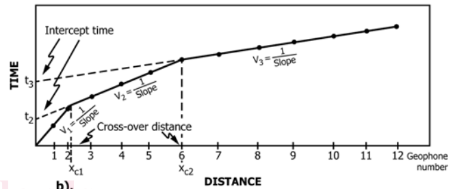
FIG. 5 (a) Seismic Raypaths and (b) Time-Distance Plot for a Three-Layer Model With Parallel Boundaries (2)
