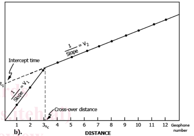
FIG. 4 (a) Seismic Raypaths and (b) Time-Distance Plot for a Two-Layer Earth With Parallel Boundaries (2)
