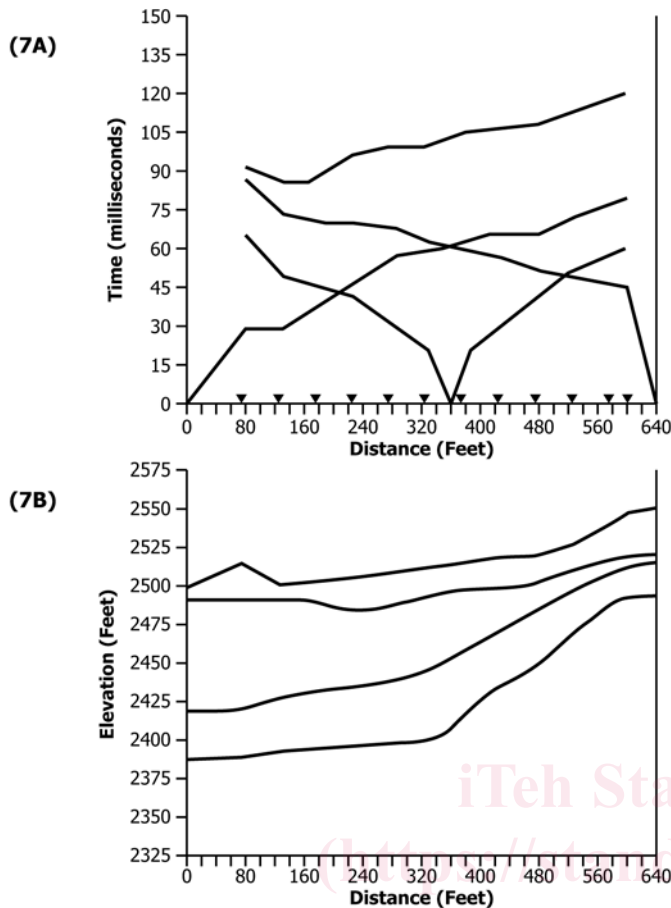
FIG. 7 Time Distance Plot (a) and Interpreted Seismic Section (b) (7)
