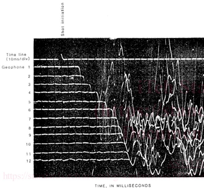
FIG. 3 Twelve-Channel Analog Seismograph Record Showing Good First Breaks Produced by an Explosive Sound Source (2)
