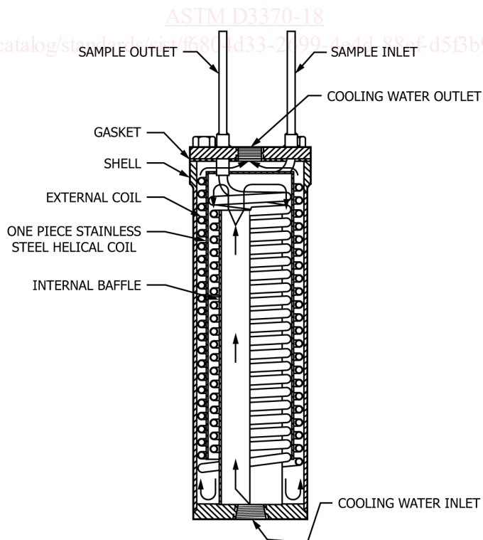
FIG. 1 Helical Coil Heat Exchanger with Removable Shell
