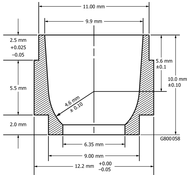
FIG. 3 Specimen Cup
