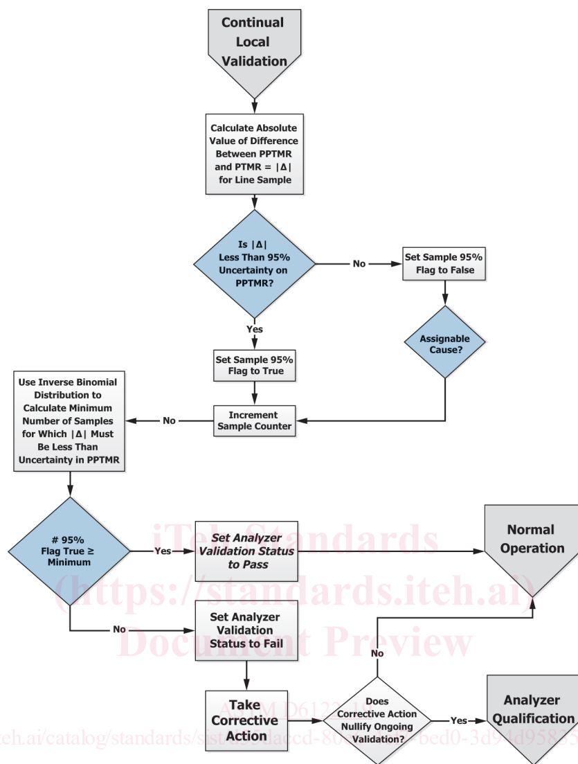
FIG. 5 Flowchart of Process Analyzer Validation Practice Continual Local Validation
