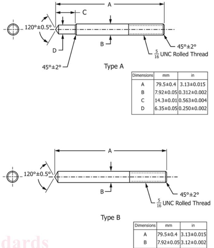
FIG. 1 Dimensions of Probes
