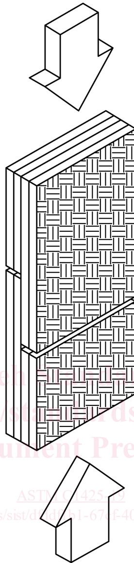
FIG. 1 Schematic of Uniaxial Compression of Double-Notched Test Specimen for the Determination of Interlaminar Shear Strength of CFCCs
