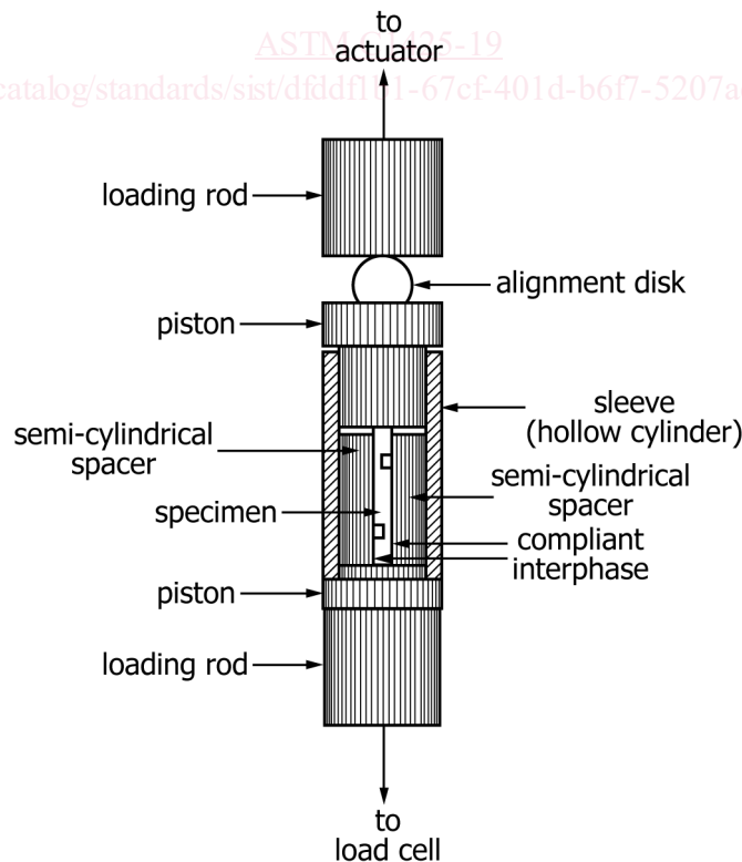
FIG. 3 Schematic of Test Fixture for the Uniaxial Compression of Double-Notched Test Specimens at Elevated Temperatures
