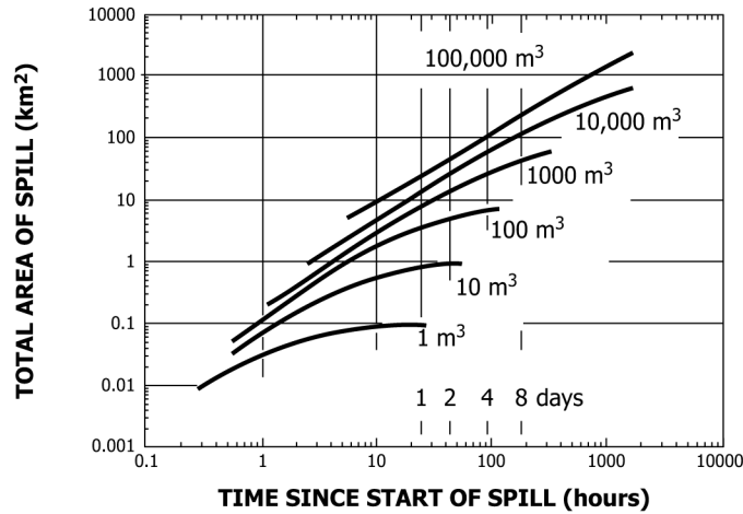
FIG. 1 Total Slick Area versus Time
