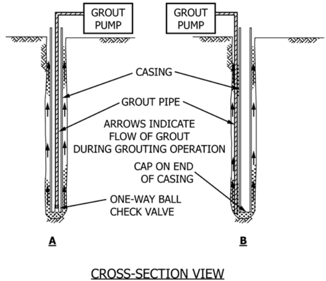
FIG. 3 Acceptable Grouting Techniques Schematic
