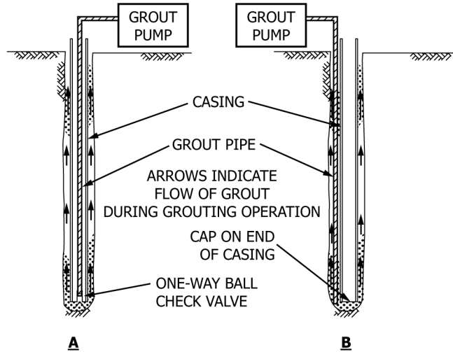
CROSS-SECTION VIEW FIG. 3 Acceptable Grouting Techniques Schematic
