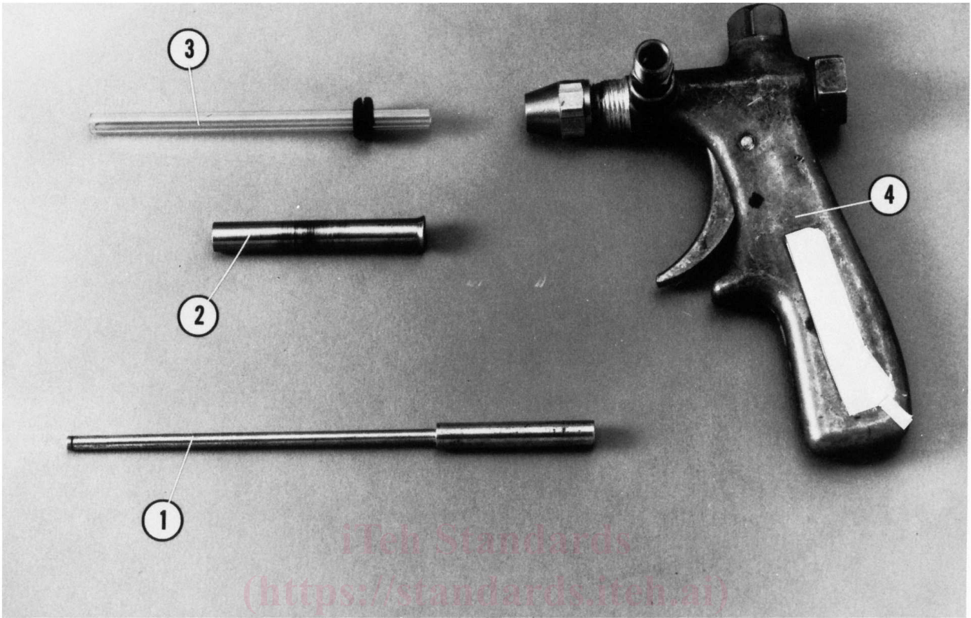
FIG. 3—Modified Modified Blast Gun Breakdown
