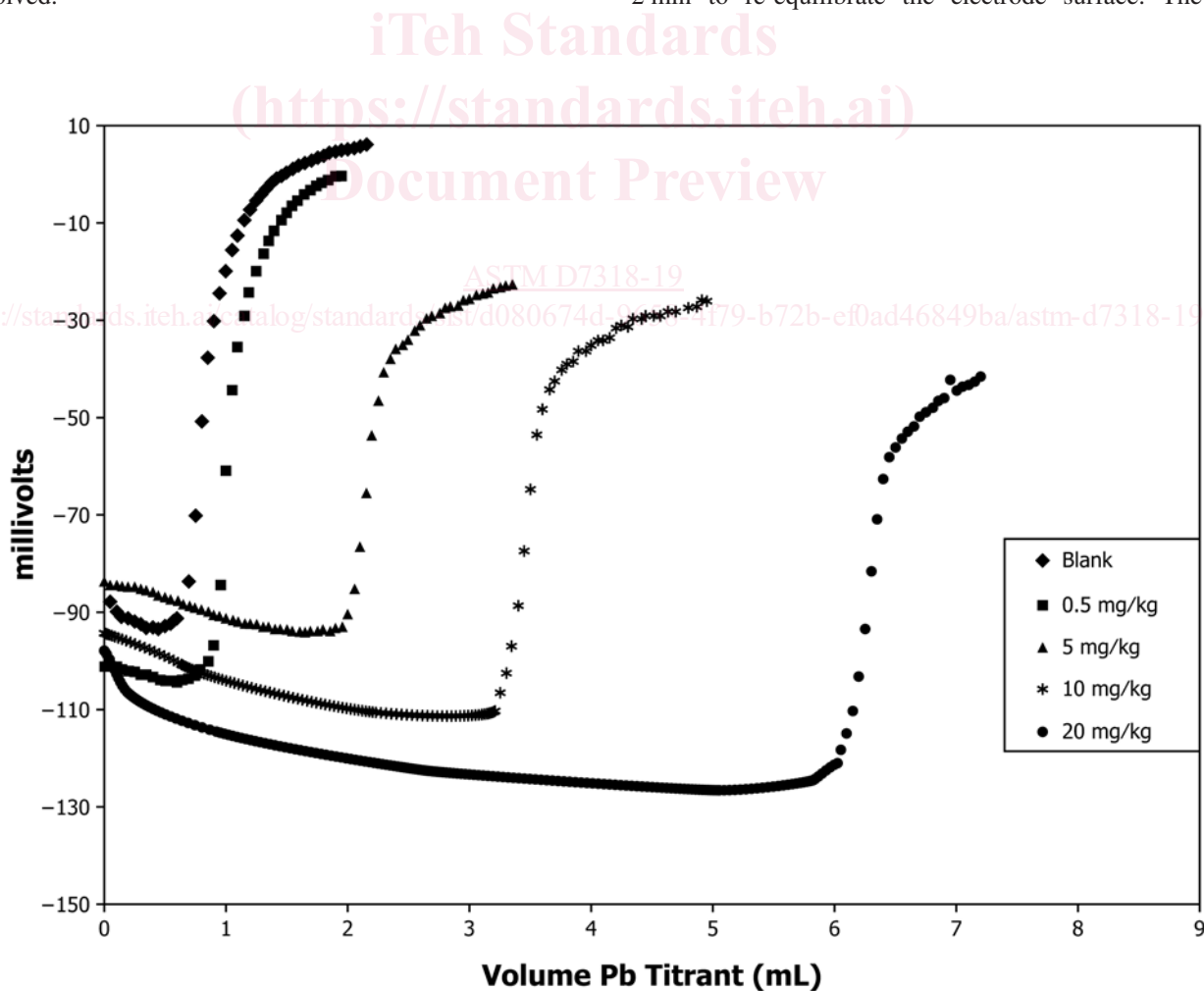
FIG. 1 Potentiometric Titration Curves for Sulfate Standards in Ethanol
