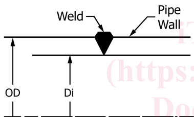
FIG. 5 Plain End Extrusion Weld
