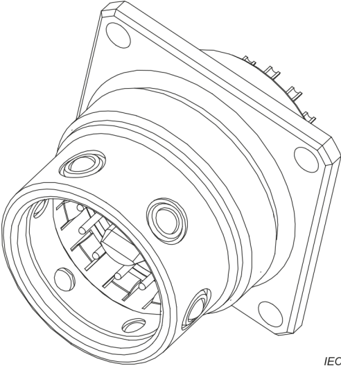
IEC Figure 2 – Fixed connector
