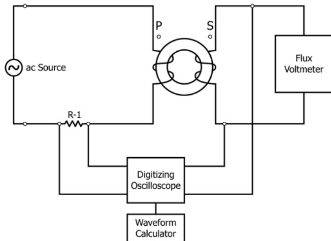
FIG. 2 Basic Circuit Diagram for Waveform Calculator Method
