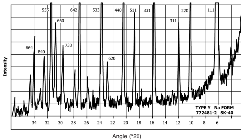
FIG. 2 NaY—Complete Diffractometer Scan Intensity
