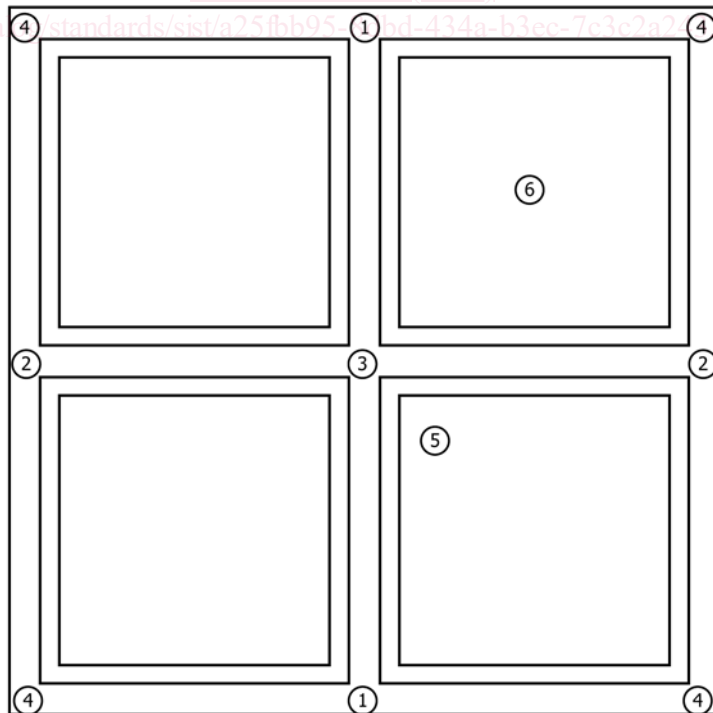
FIG. 1 Test Assembly Elevation Location of Strike Points Described in Table 1
