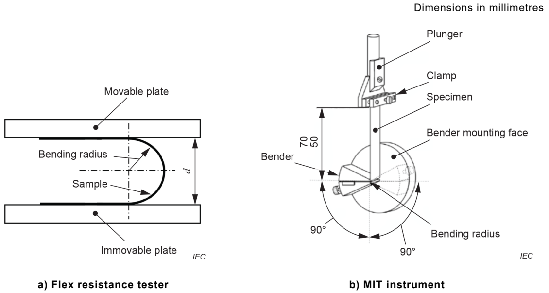
Figure 1 – Bending apparatuses of IEC 62899-201
