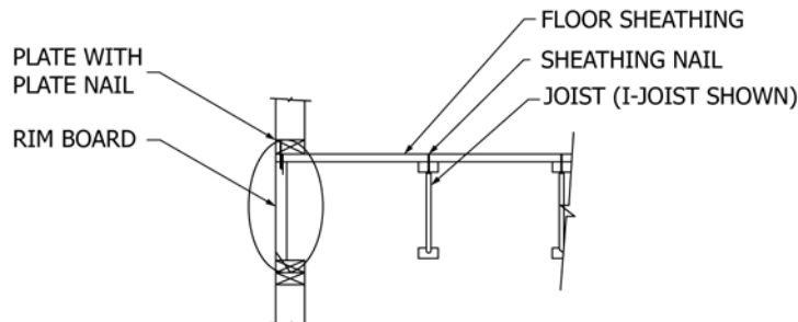
b.) Parallel to the joists
