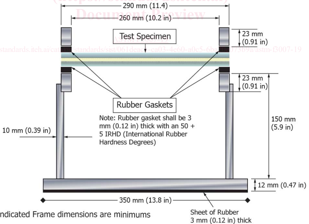
FIG. 1 Holding Fixture for Drop Test – Cut-away Side View
