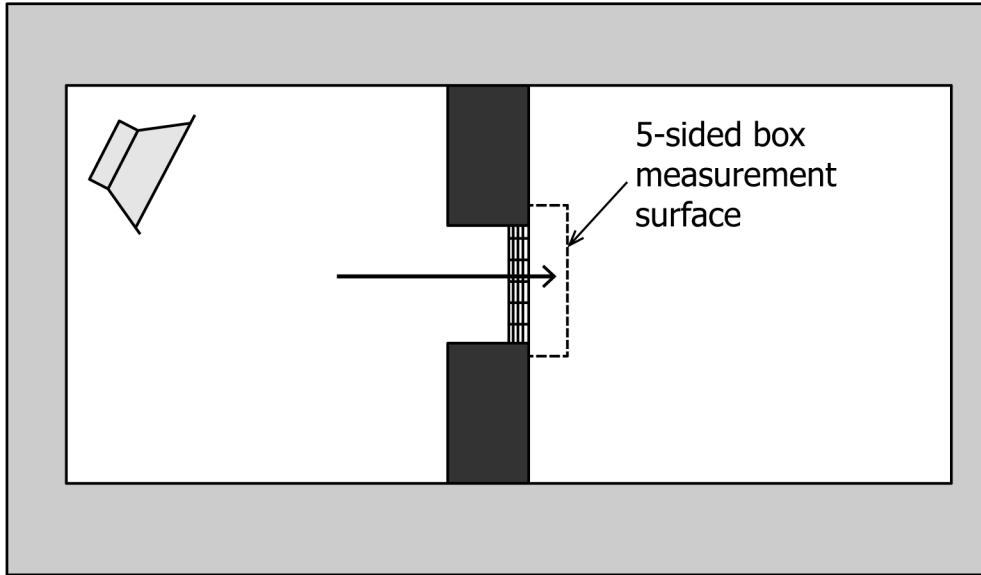
FIG. 4 Measurement Surface – Specimen Mounted in Larger Partition
