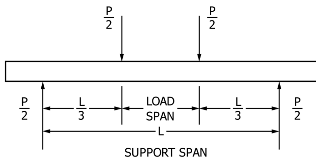
FIG. 1 Loading Diagram
