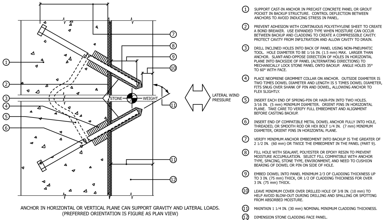
FIG. 6 Cast-In Anchors
