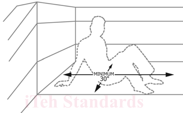
FIG. 12 Slide Landing Transition Area
