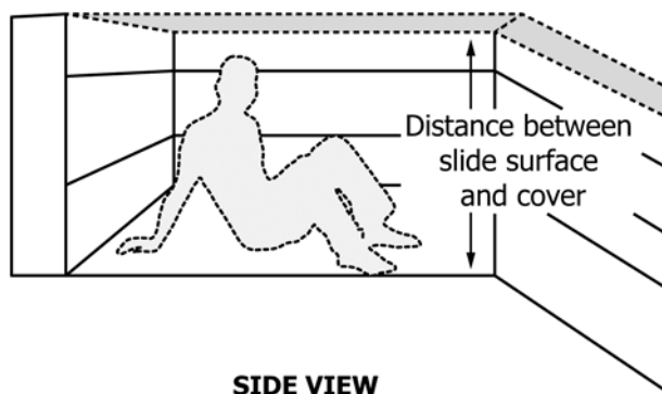
SIDE VIEW FIG. 9 Clearance Between Slide Surface and Protective Cover
