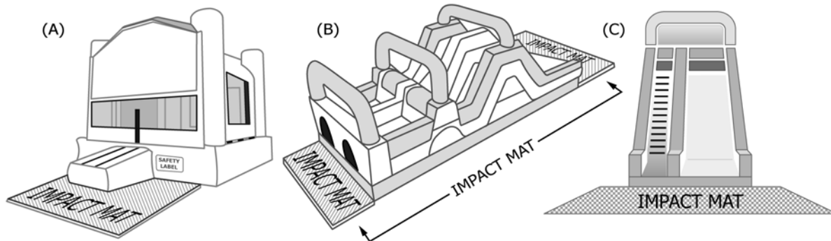
FIG. 10 Examples of Impact Mat Placement
