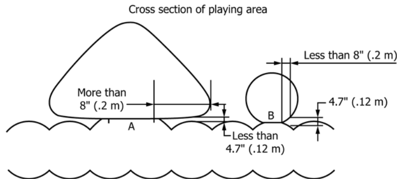
The large slide fixed at A forms an entrapment point. The ball fixed at point B does not form an entrapment point.
