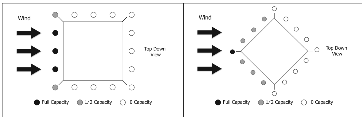
FIG. 4 Anchor Effectiveness
