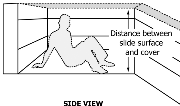
FIG. 9 Clearance Between Slide Surface and Protective Cover
