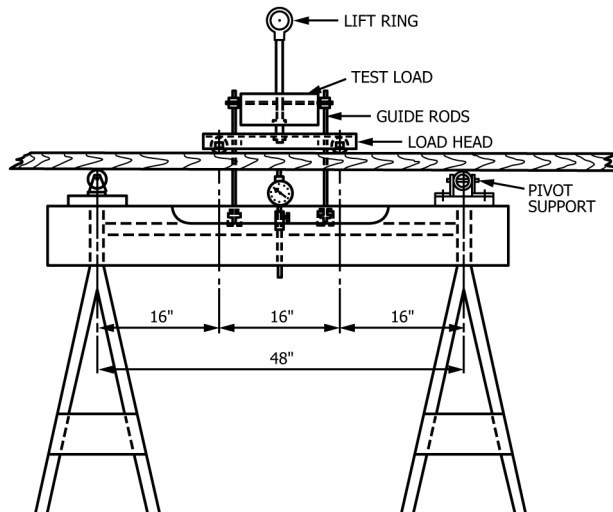
FIG. 1 Schematic of Static Third-Point Bending Testing Device
