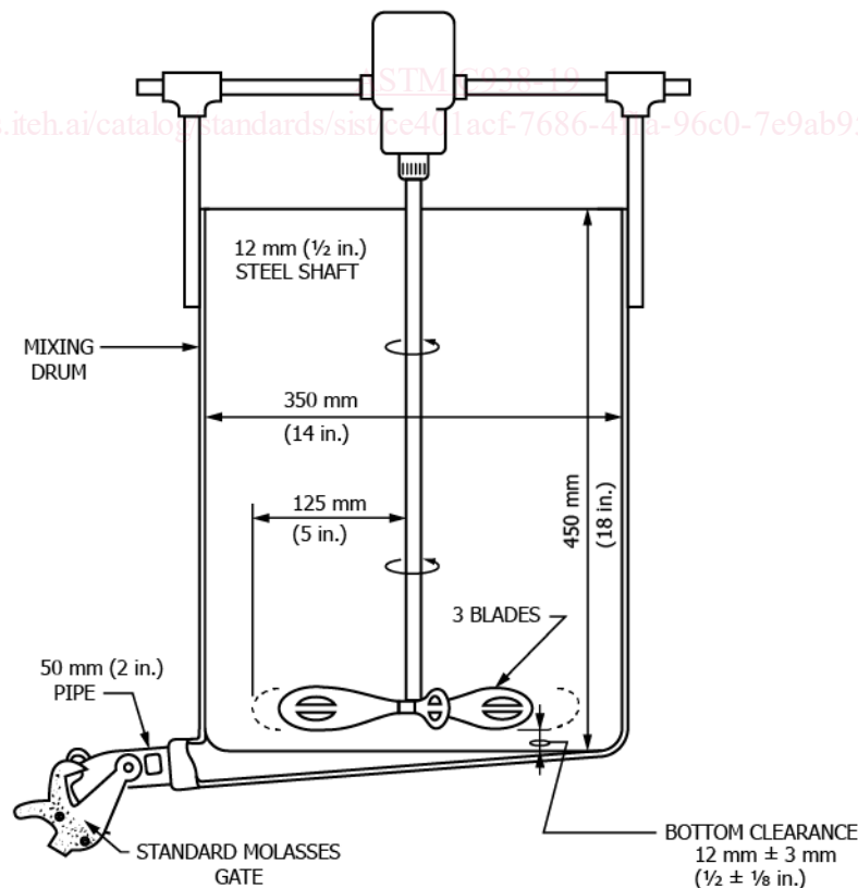
FIG. 1 Grout Mixer
