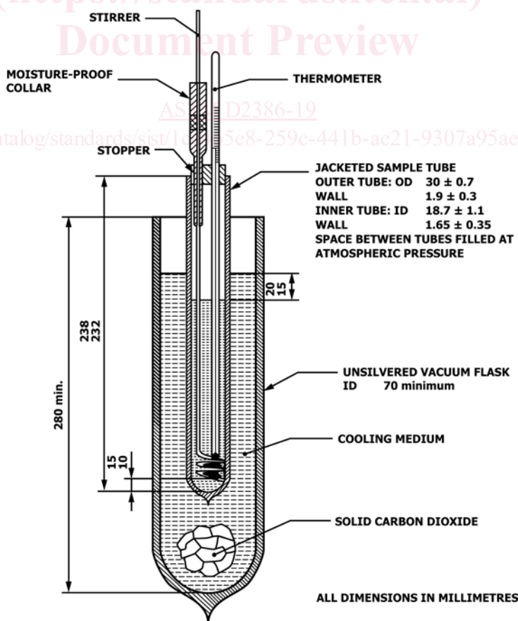
FIG. 1 Freezing Point Apparatus
