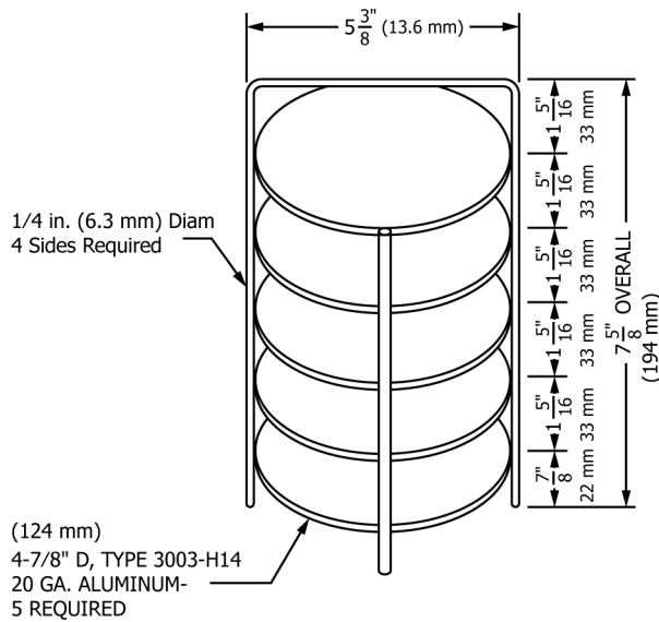
FIG. 2 SSG Samples Sintering Rack
