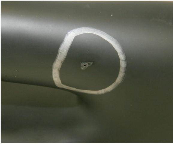
FIG. 6 Breakdown (Dielectric Failure)
