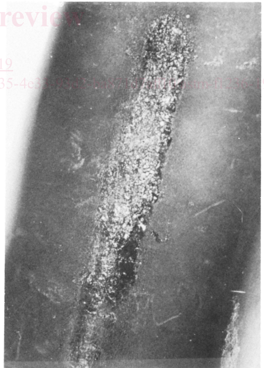
FIG. 18 Hard Spot
