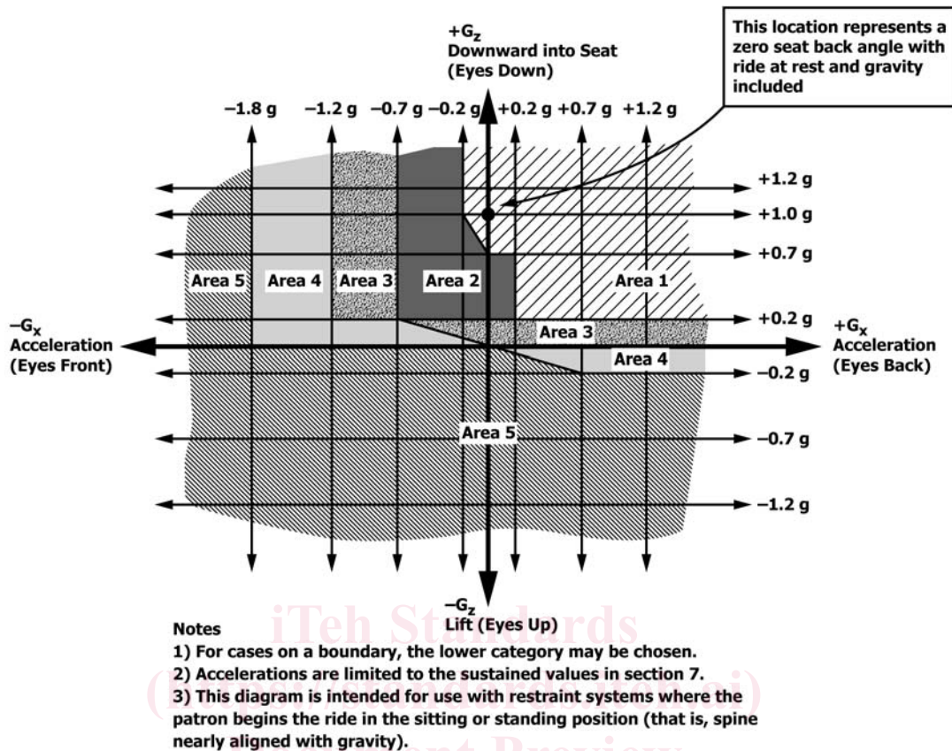
FIG. 2 Restraint Determination Diagram—Accelerations in Design Stage
