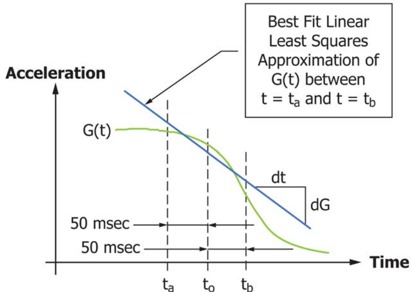
FIG. 9 Onset Calculation
