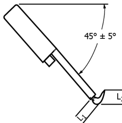
FIG. 4 Position of Specimen for the Flame Height Measurement Described in 8.2.3.4
