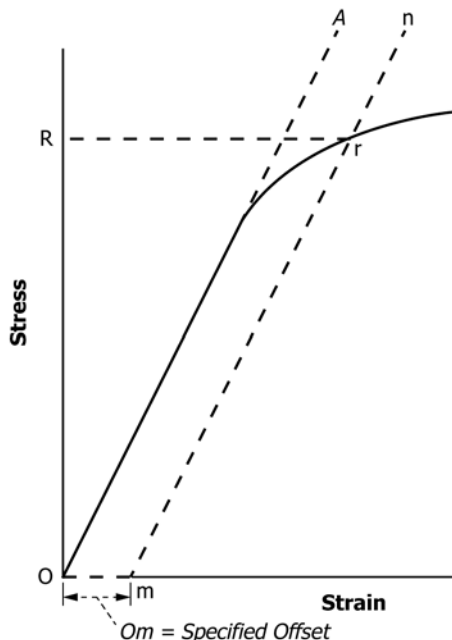
FIG. 1 Stress-Strain Diagram for Determination of Yield Strength by the Offset Method
