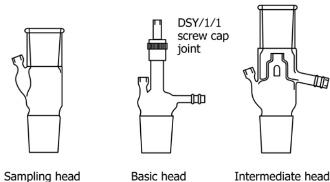
FIG. 3 Basic Head
