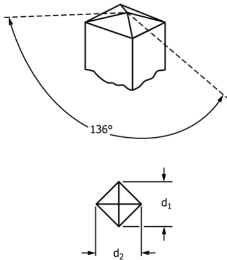
FIG. 2 Vickers Indenter
