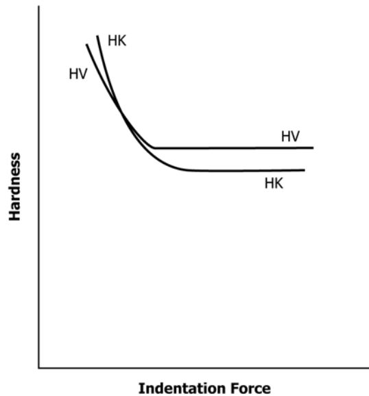
FIG. 1 Indentation Size Effect (ISE) Curves for a Ceramic (Sometimes they continuously approach a plateau hardness at larger forces, but sometimes they can have a shift or step if cracking occurs)
