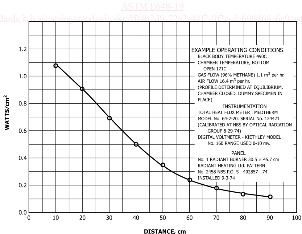
FIG. 2 Standard Radiant Heat Energy Flux Profile
